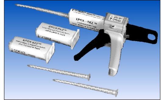
Applicator Gun With Disposable Cartridges & Mixer Sticks
